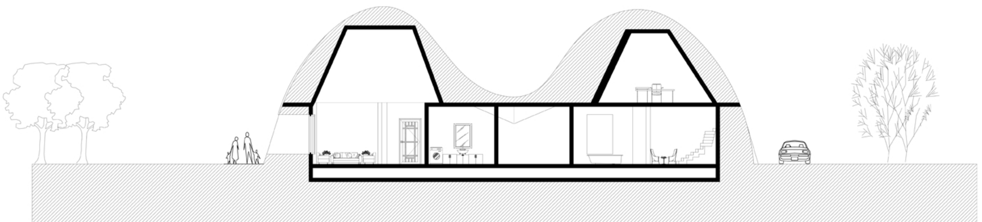
section dd'
